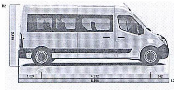
L3H2 EXECUTIVE / VIP: CHASSI LONGO
